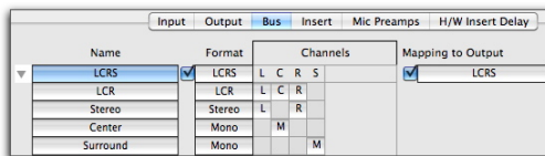
Bus page, LCRS output bus with sub-paths
